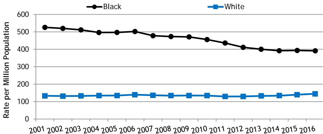
Figure 68. Adjusted incident rates of end stage renal disease (ESRD) due to diabetes per million population, 2001-2016
